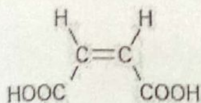
Maleic acid
