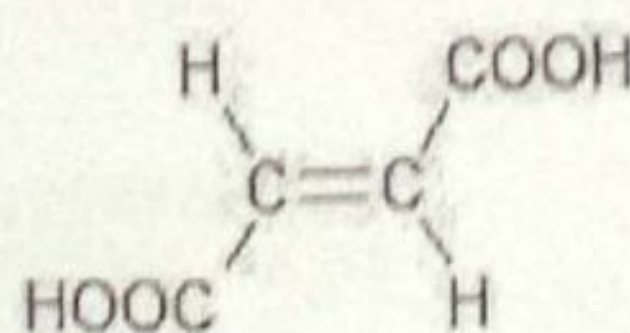
Fumaric acid
